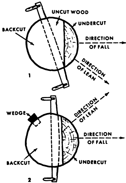
1 HOLDING A CORNER IN SAWING A LEANING TREE 2 USE OF WEDGES ON A LEANING TREE
